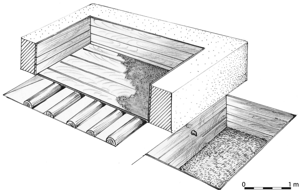
Figure 12. Reconstruction of a leaching pit according to archaeological and ethnographic data (Drawing by Wang Xinsheng).
